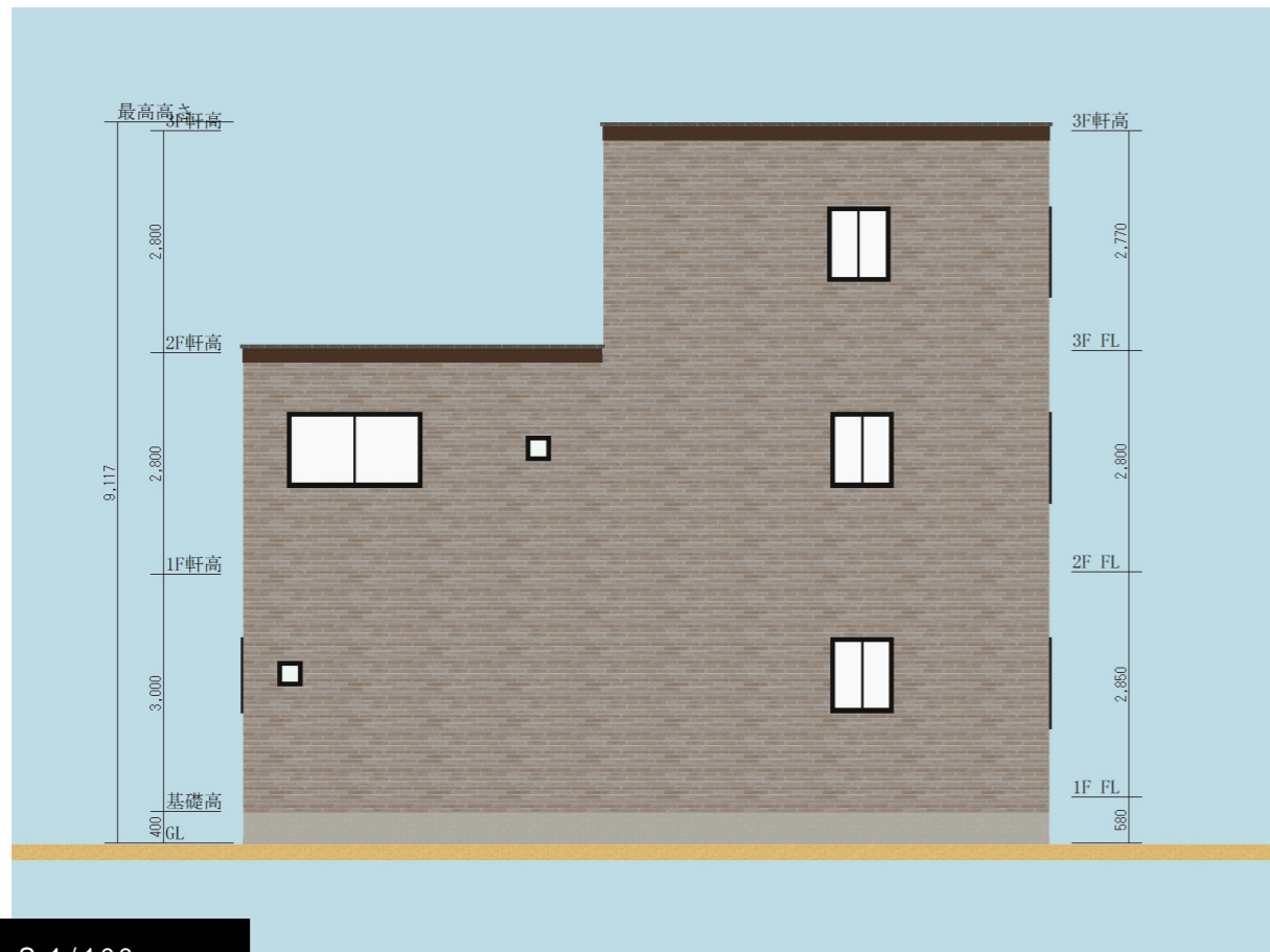
NORTH S:1/100
