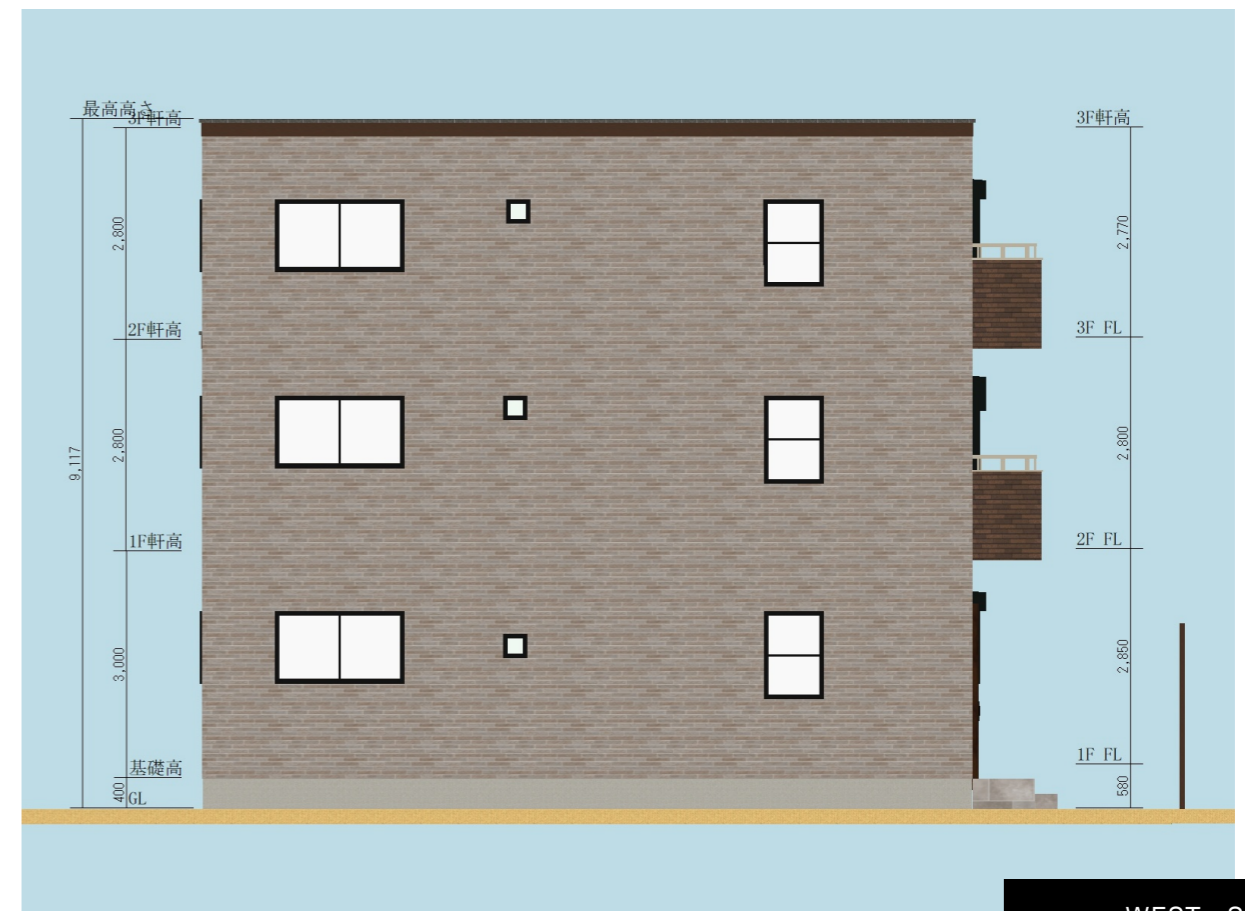
WEST S:1/100
