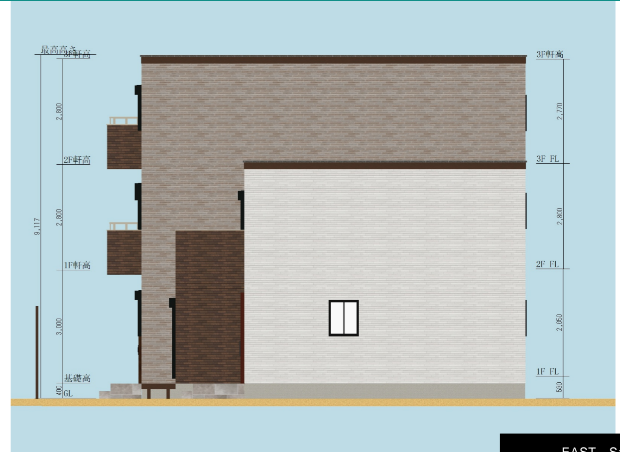
EAST S:1/100
