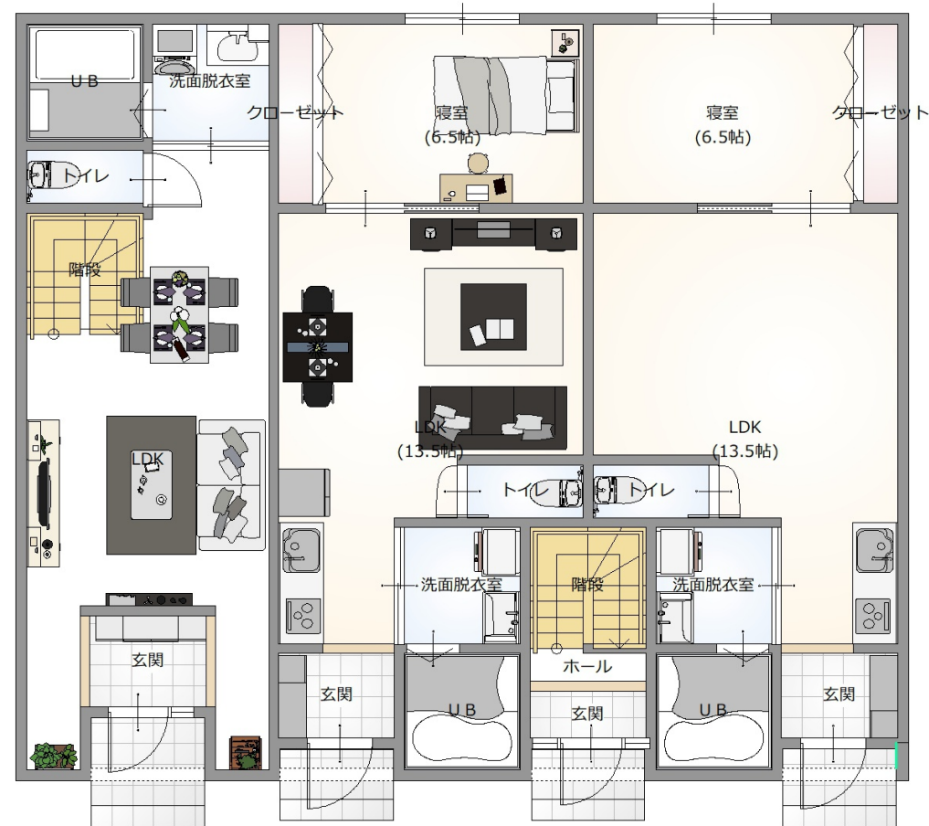
1st FLOOR
