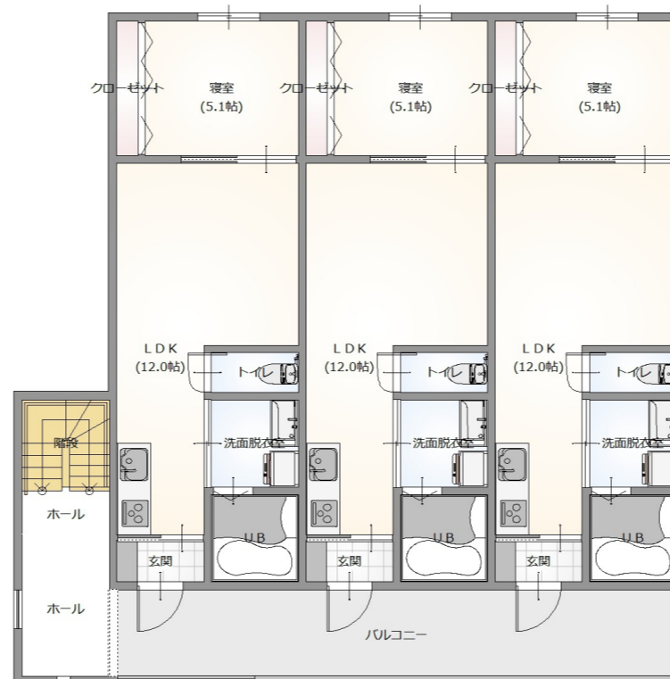
2nd FLOOR
