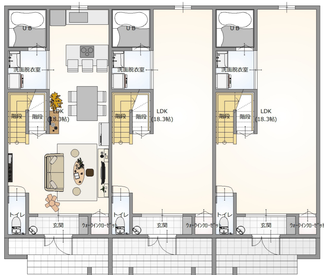
1st FLOOR
