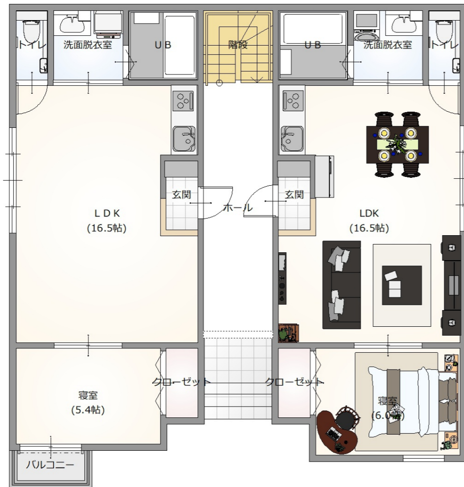
1st FLOOR
