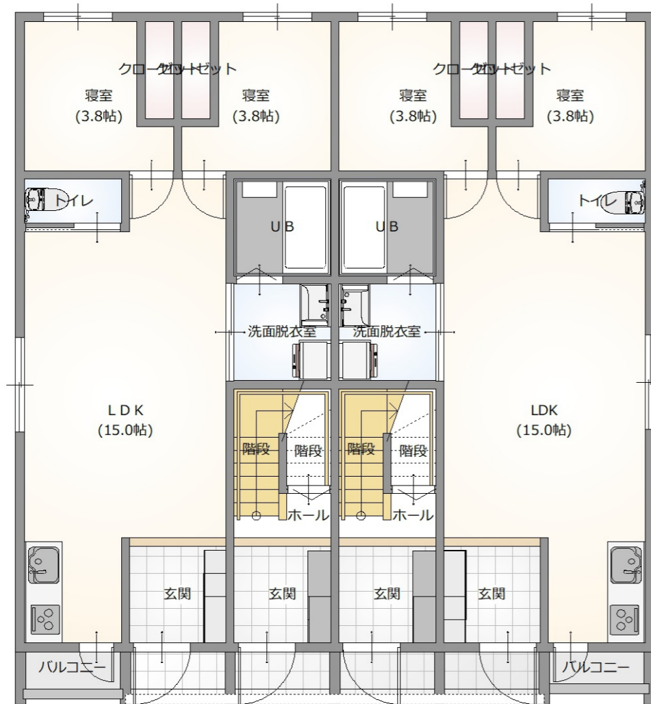
1st FLOOR
