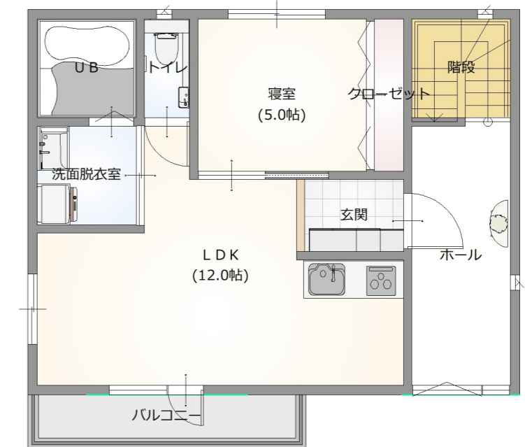
3rd FLOOR S:1/100
