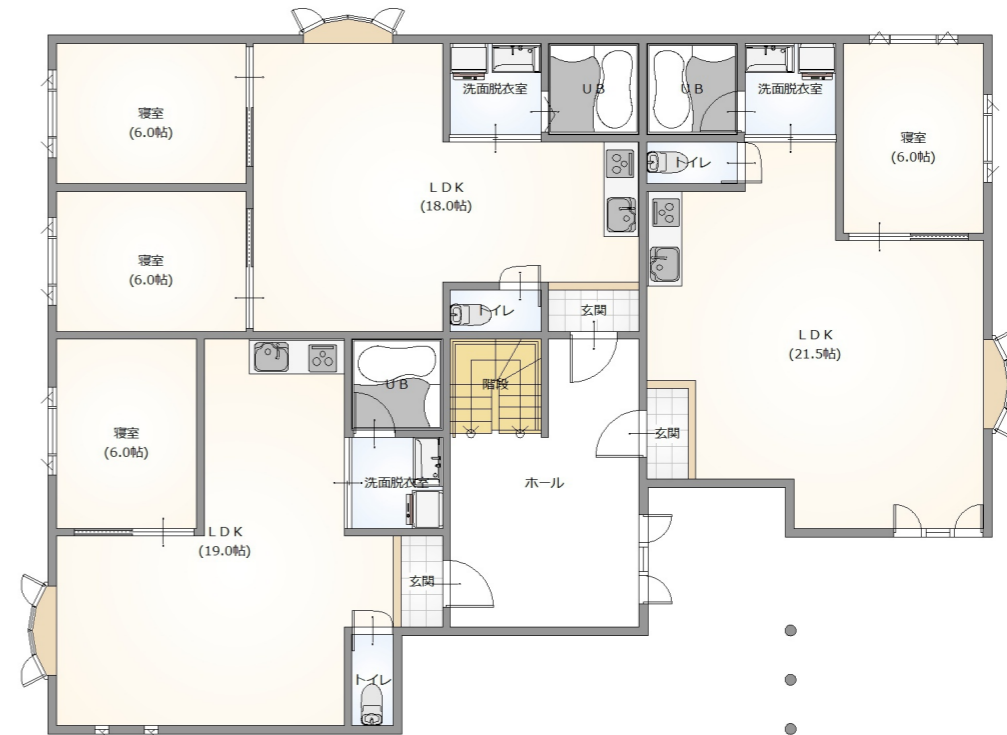
2nd FLOOR S:1/100
