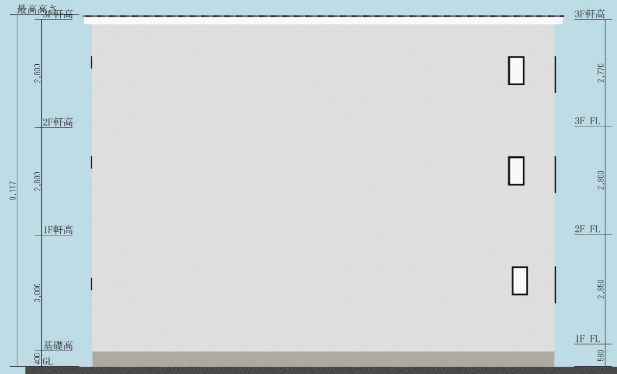
NORTH S:1/100
