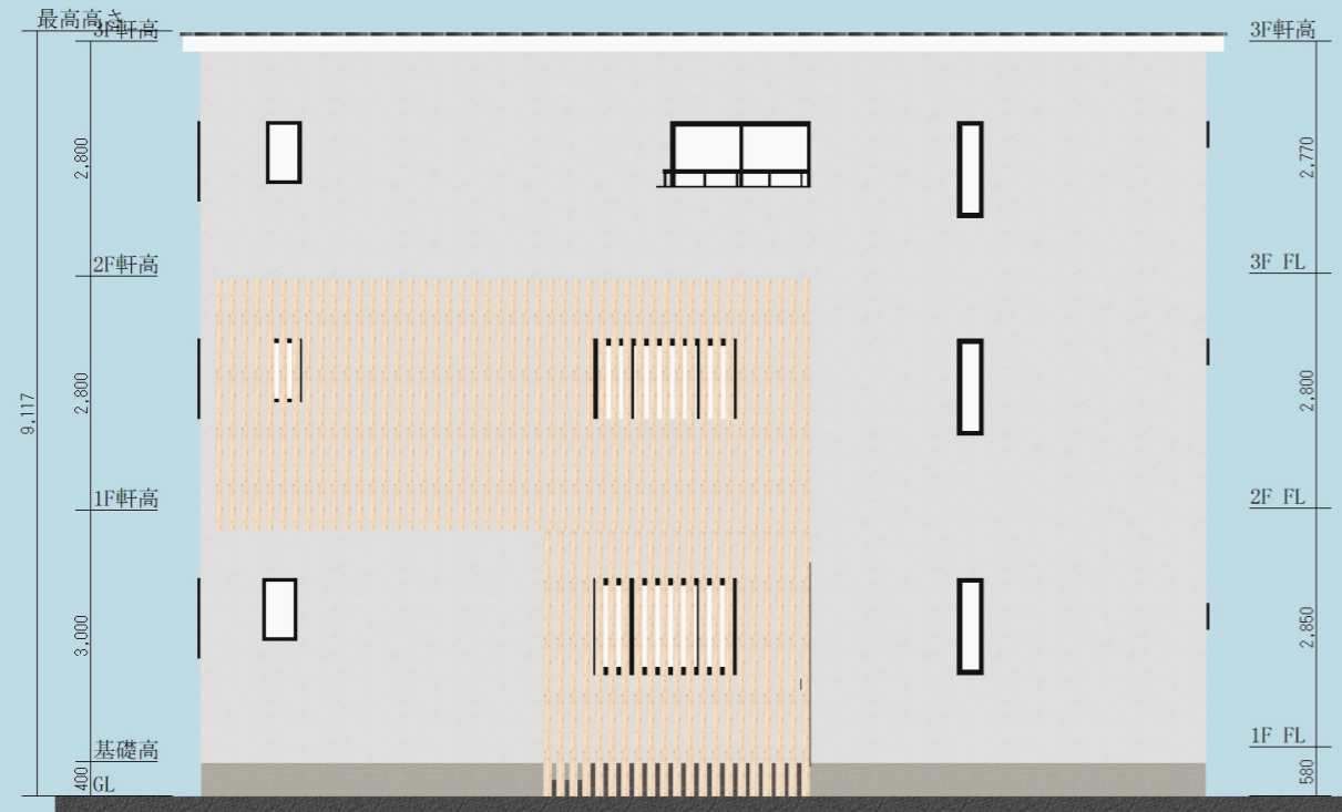
SOUTH S:1/100
