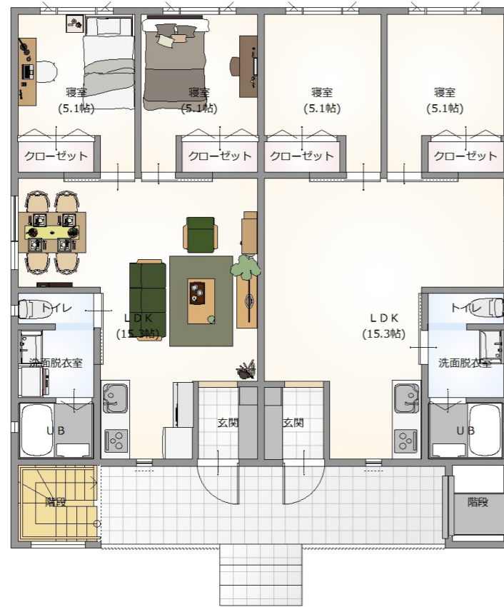
1st FLOOR
