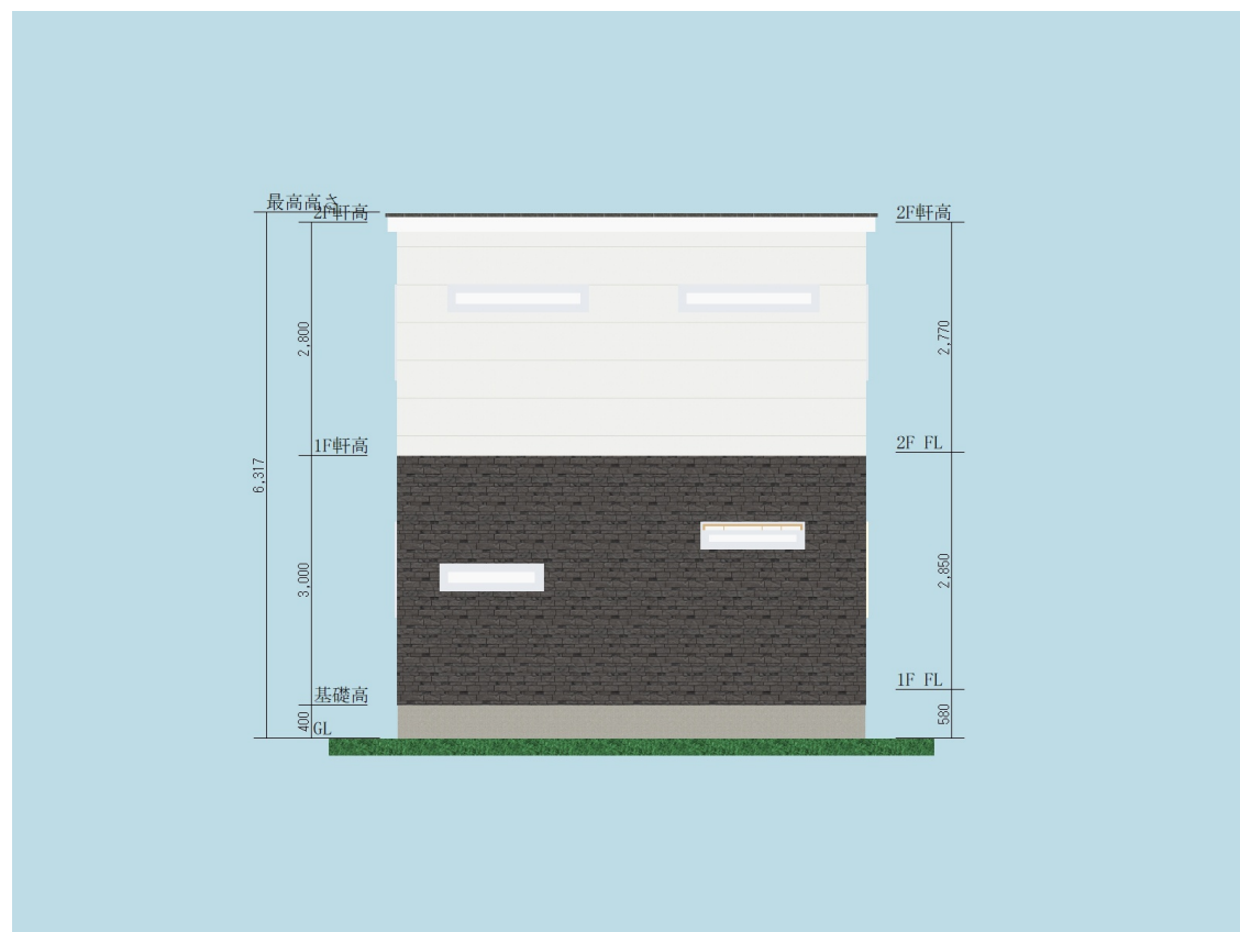
NORTH S:1/100
