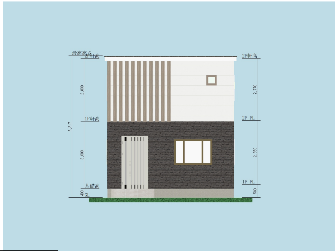
SOUTH S:1/100
