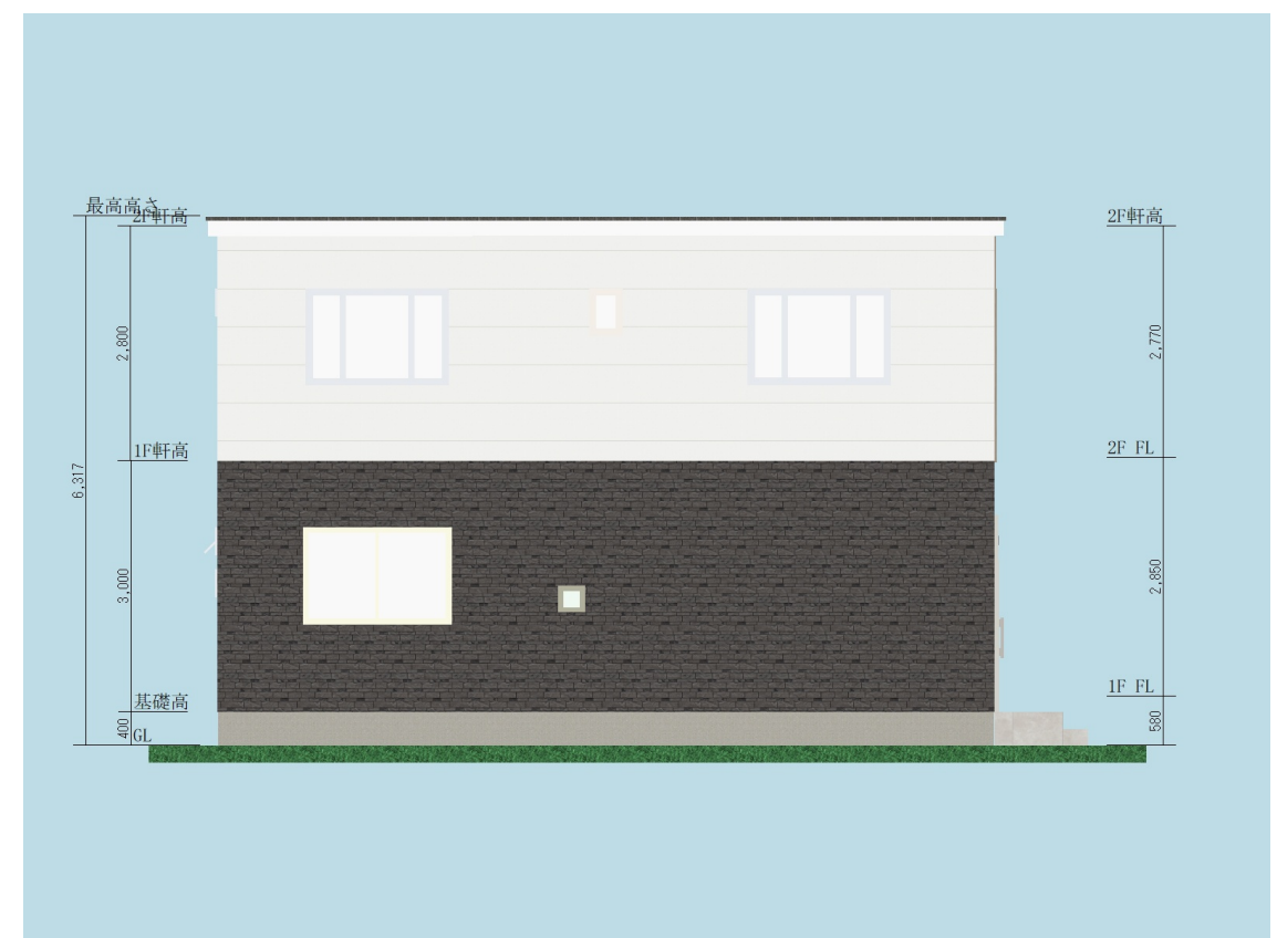
WEST S:1/100
